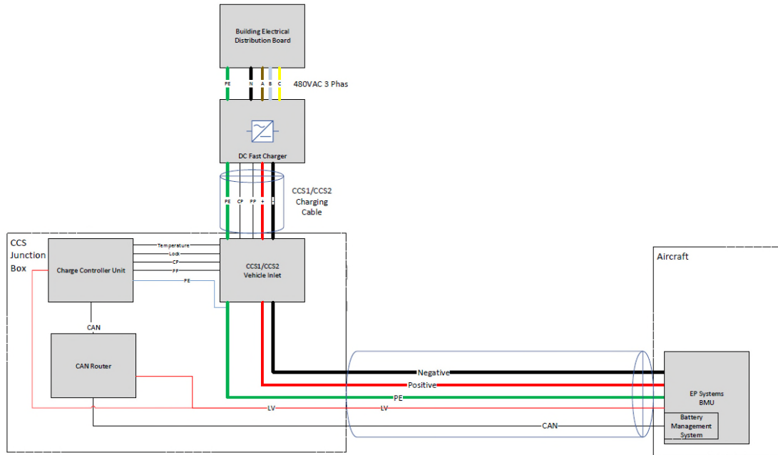
Fig. 19 ESS Charging System
