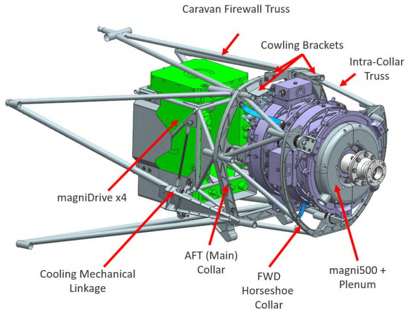
Fig. 6 magniX EPU Integration
