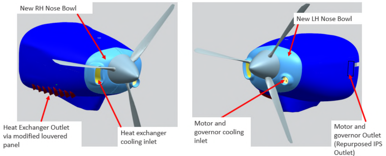
Fig. 8 Custom Nose Bowl and Mounts
