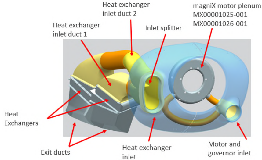
Fig. 9 Custom Ducting
