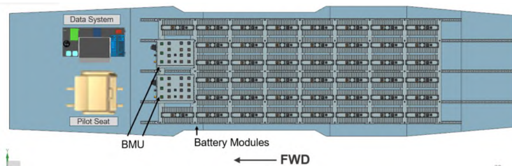
Fig. 5 ESS Cabin Layout
