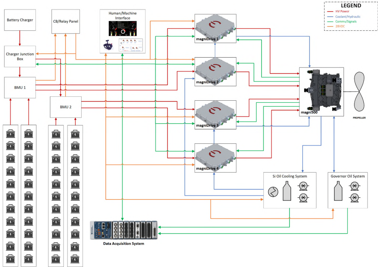
Fig. 2 Electric Power Train System Architecture
