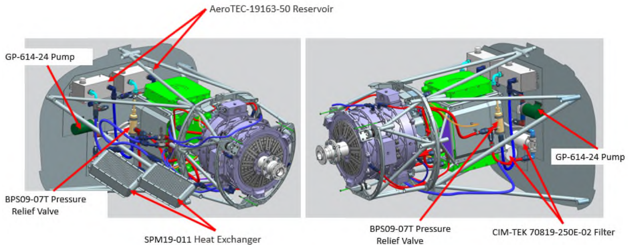
Fig. 7 Cooling System Installation Layout
