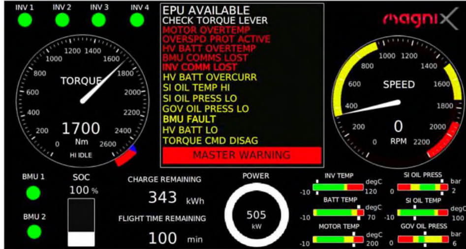
Fig. 12 Overview of the Flight Deck Engine Display
